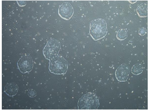
CiRA-j-1503-D: passage-3
